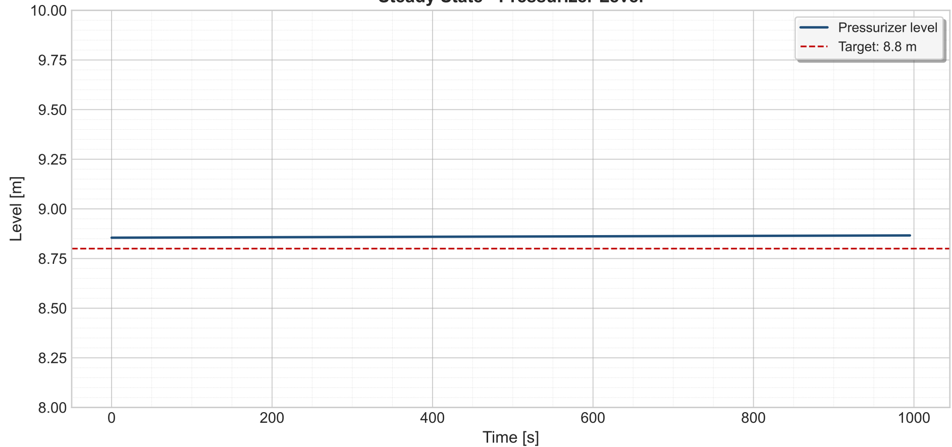
Steady State - Pressurizer Level
